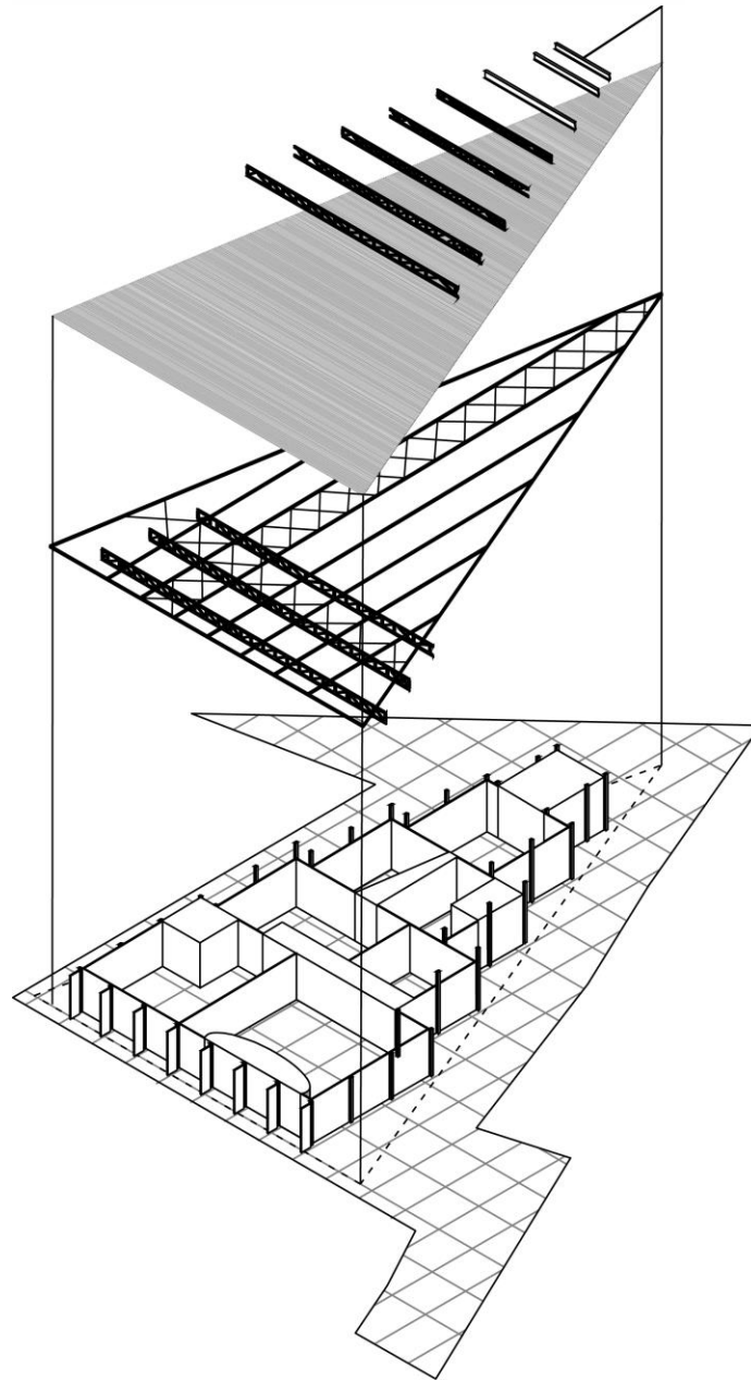
EXPLODED VIEW
